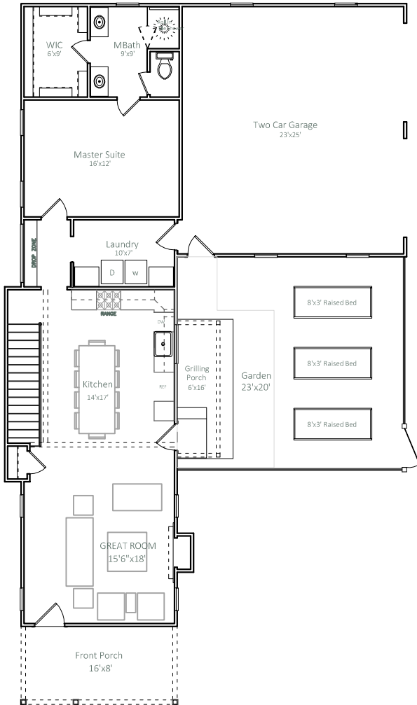
MAIN FLOOR 1073 S.F.
